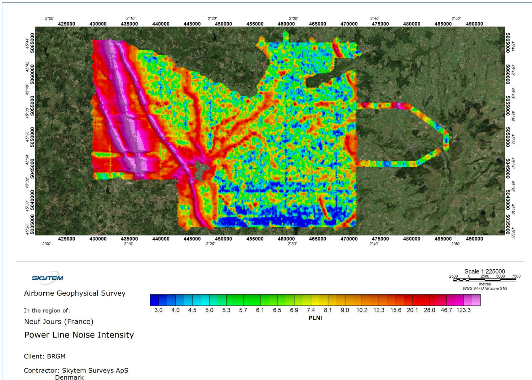
Figure 17. Power line noise intensity SkyTEM Survey Neuf Jours – December 2023
