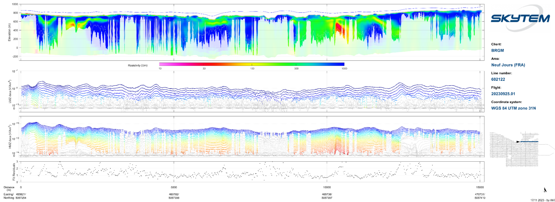
Figure 20 Example of section plot from the inversion of SkyTEM306HPM data. From top to bottom: conductivity section with flight height and Depth of Investigation (DOI), LM and HM gate plot (data=dots, model=line), residual.
